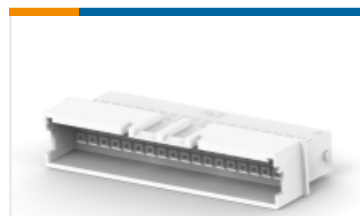
TE Part # 3-2324201-8 HSG,REC,FREE-HANGING,GWT, DUALROW,EP2.5
